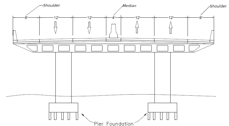
TYPICAL SECTION
