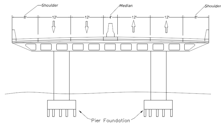
TYPICAL SECTION
