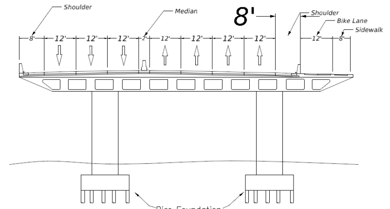
Pier Foundation TYPICAL SECTION
