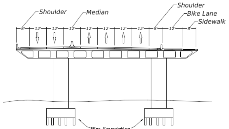
TYPICAL SECTION
